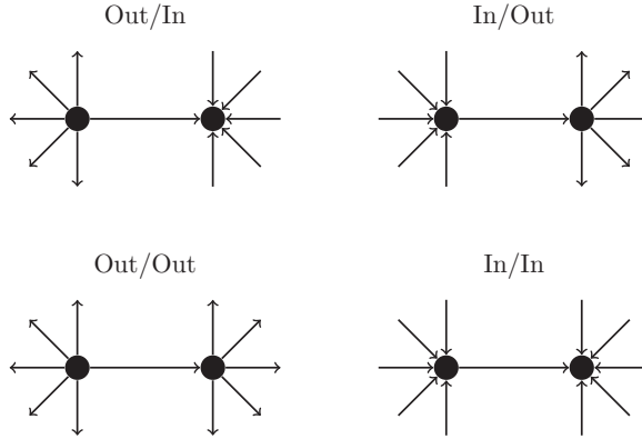
Figure 1 Four degree-degree dependency types.
