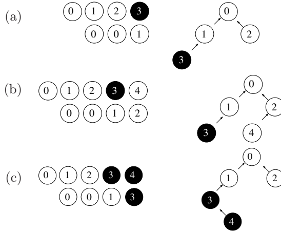
Figure 1. Illustration of the urn model: (a) Growing network after three steps. We choose to follow the subtree T_3 . (b) Node 4 is not linked to T_3 . (c) Node 4 is linked to T_3 .
