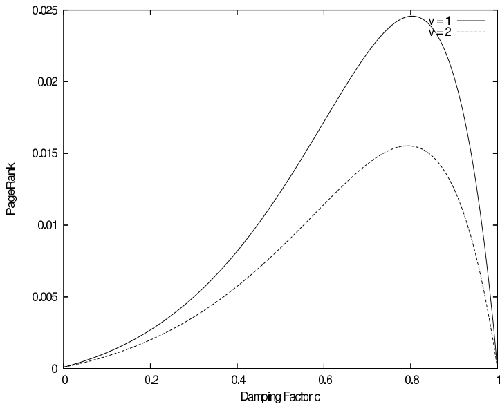
Figure 5. The expected value of PageRank as a function of c for v = 1, 2 and n = 10000 .
