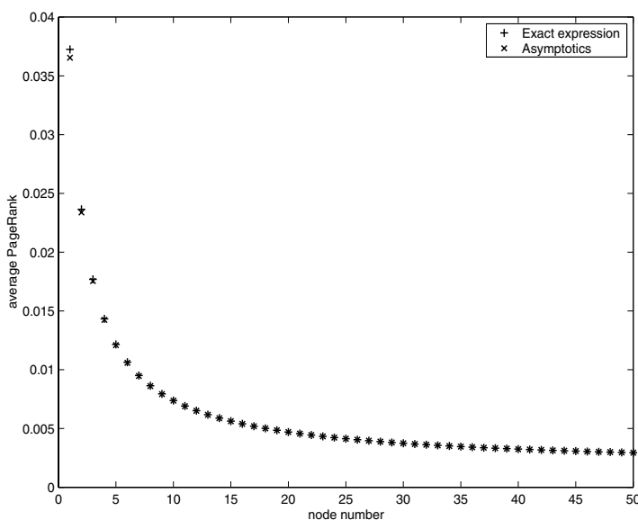
Figure 2. Comparison between the asymptotics (7.6) and the exact expression (7.1).
